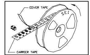
Tape-and-Reel Option
